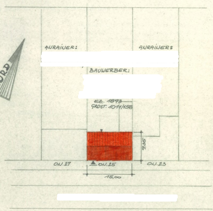
LAGEPLAN MS. 1:500
